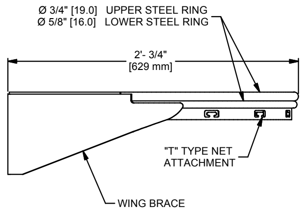
WING BRACE
